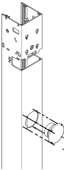
Couple Pole - Front
