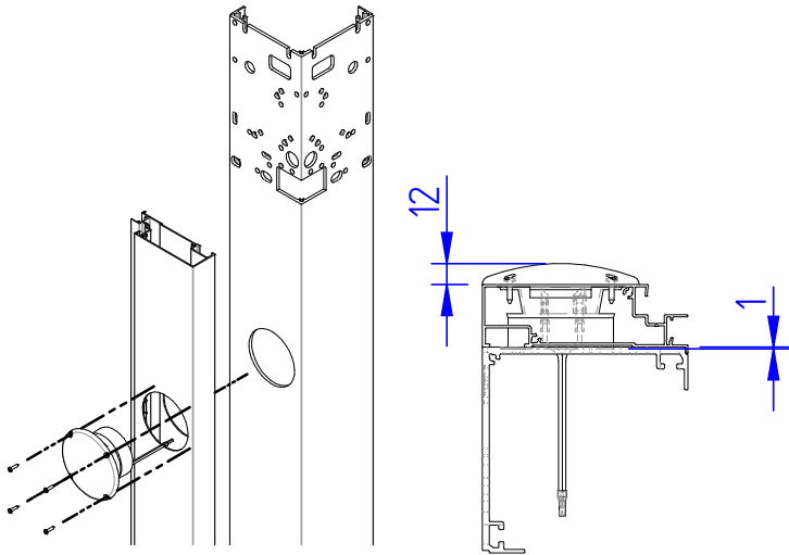
Vertical Pole - With Screen
