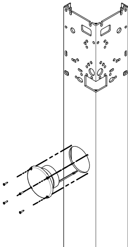
Vertical Pole - No Screen
