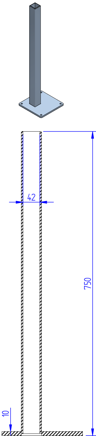
SECTION B-B
